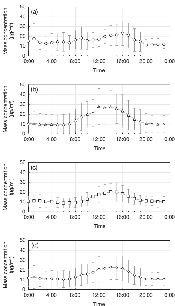
Fig. 2. Diurnal variation of \text{PM}_{2.5} mass concentration measured using the SHARP in 24-hour continuous measurements conducted in 2014. (a) Hourly mean values in spring (March to May), (b) summer (June to August), (c) fall (September to November), and (d) across all seasons. Error bars show one standard deviation.
