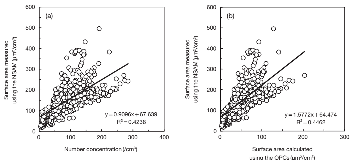
Fig. 6. Comparisons between PM 2.5 surface area concentration measured using the NSAM and PM 2.5 number and surface area concentrations measured using the OPC in 24-hour continuous measurements: (a) number concentration measured using the OPC and (b) surface area concentration calculated using the number concentration of the OPC. The measurements were carried out from July to November, 2014.
