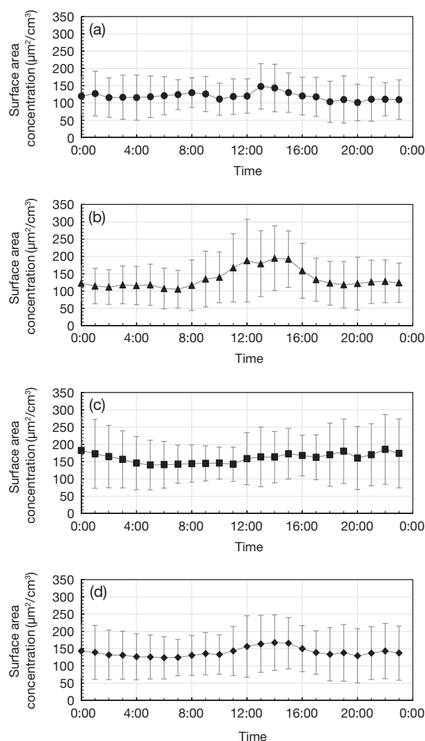
Fig. 3. Diurnal variation of \text{PM}_{2.5} surface area concentration measured using the NSAM in 24-hour continuous measurements conducted in 2014. (a) Hourly mean values in spring (March to May), (b) summer (June to August), (c) fall (September to November), and (d) across all seasons. Error bars show one standard deviation.
