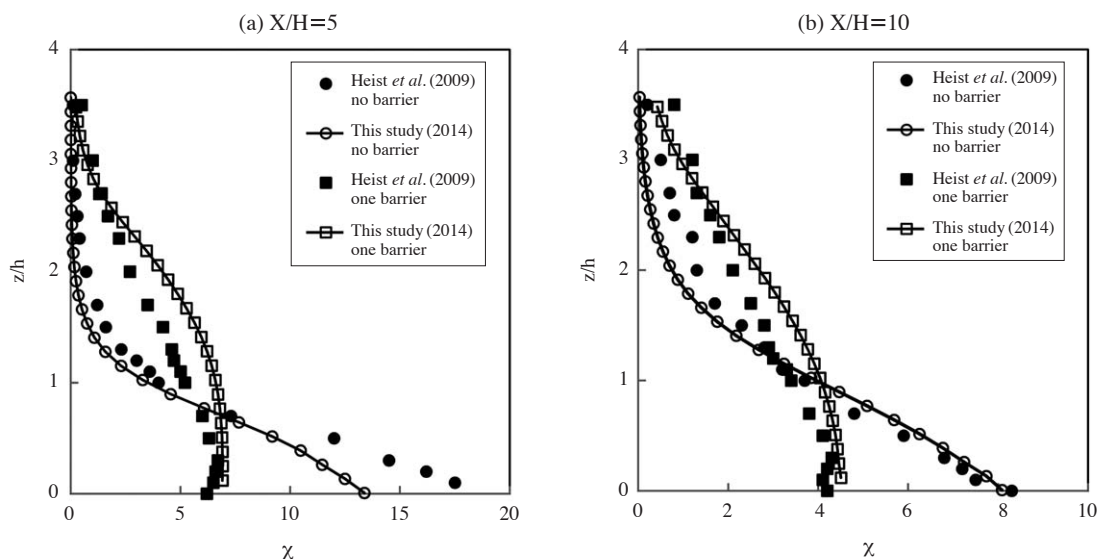
Fig. 2. Comparison of experimental with CFD concentration profiles of no and one barrier cases at (a) x/h=5, (b) x/h=10.
