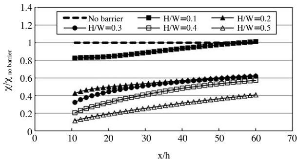
Fig. 7. Leeward surface ( z=1 m) concentrations of various height-to-street-width aspect ratio double-noise barrier cases.
