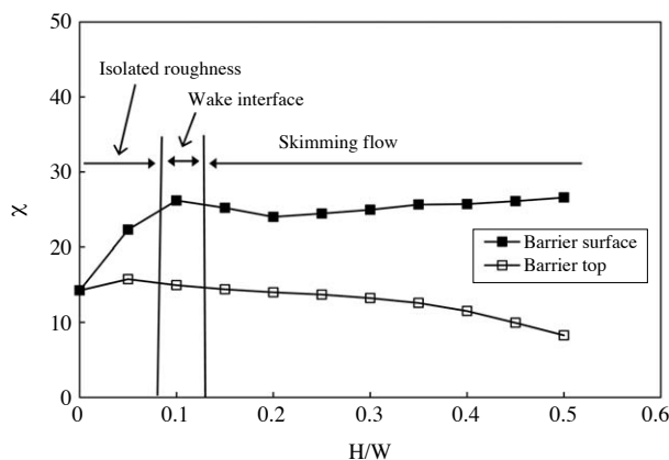
Fig. 6. Flow regime and normalized average concentrations of barrier surface ( z=1 m) and barrier top (from 2 to 20 m) of inner region of double-noise barriers.
